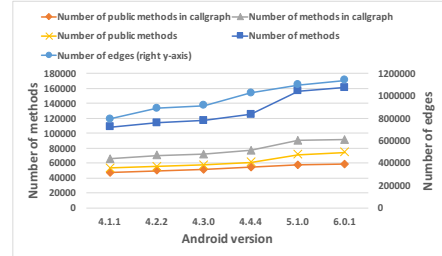
Fig. 3. Numbers of Methods and Edges
